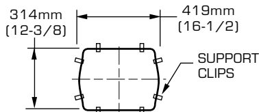
MODEL 7182.000
