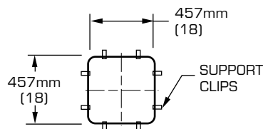
MODEL 7185
