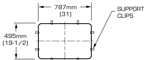
MODEL 7103
