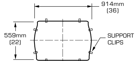
MODEL 7255
