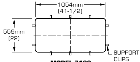
MODEL 7183
