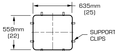
MODEL 7172
