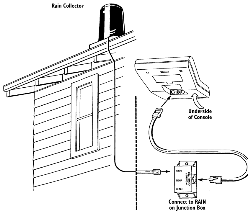
Typical Installation
