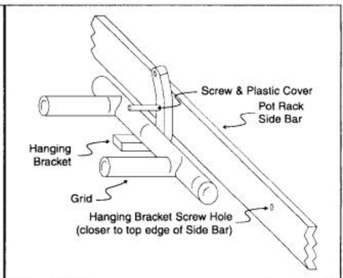
Figure 2 Hanging Bracket Installation
